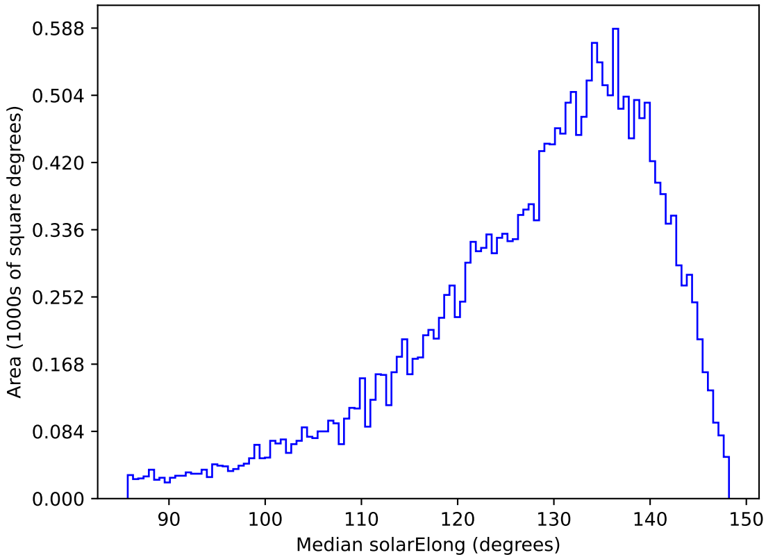
mw_roll_bulge_v3.3_10yrs All sky y band: Median solarElong
