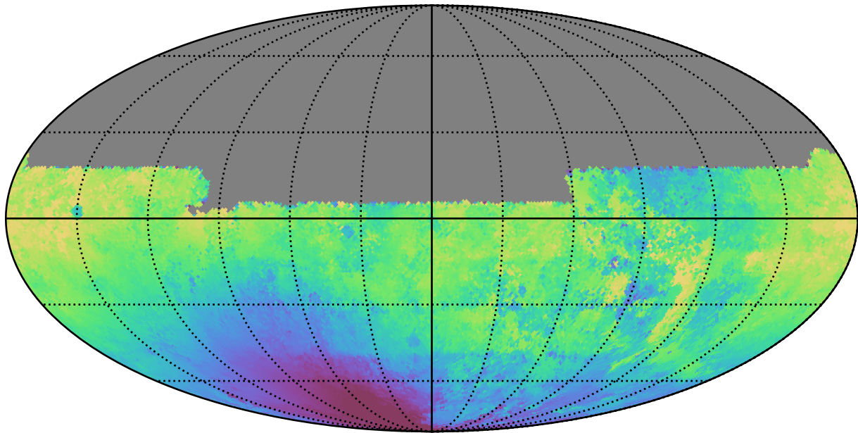
mw_roll_bulge_v3.3_10yrs All sky u band: Median solarElong
