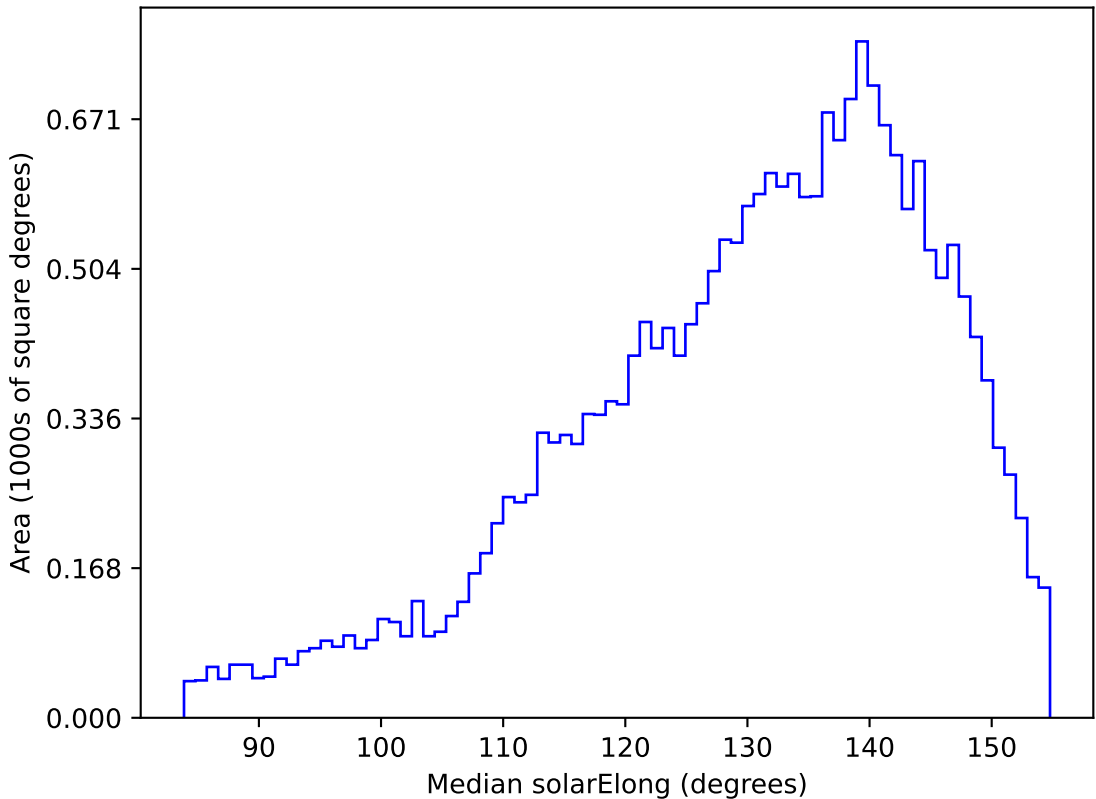
mw_roll_bulge_v3.3_10yrs All sky u band: Median solarElong
