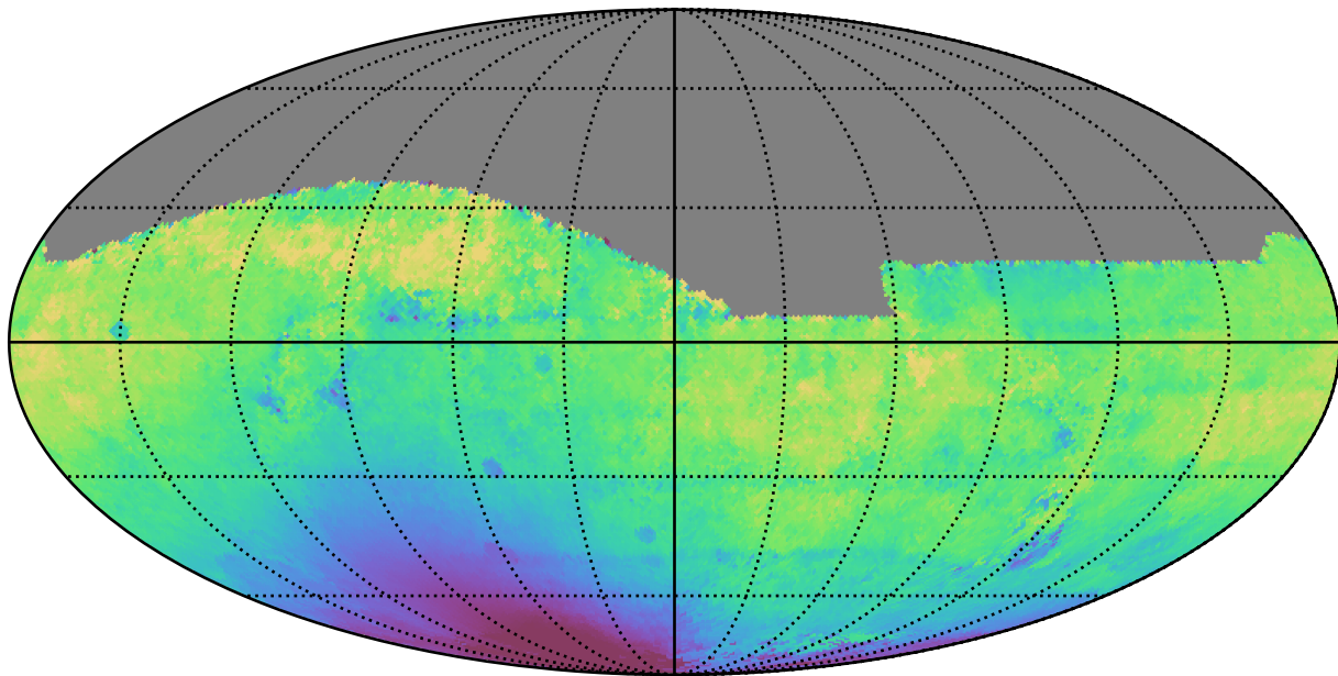
mw_roll_bulge_v3.3_10yrs All sky i band: Median solarElong
