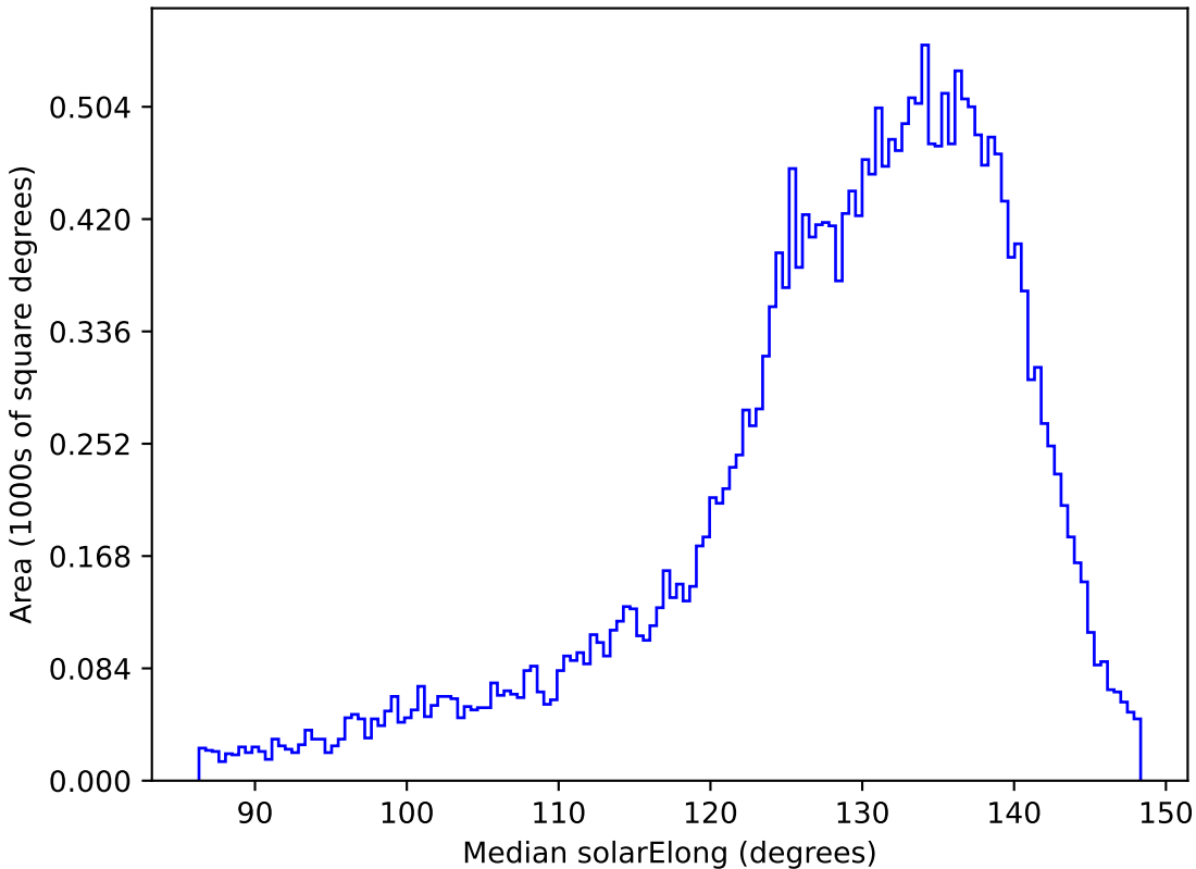
mw_roll_bulge_v3.3_10yrs All sky i band: Median solarElong
