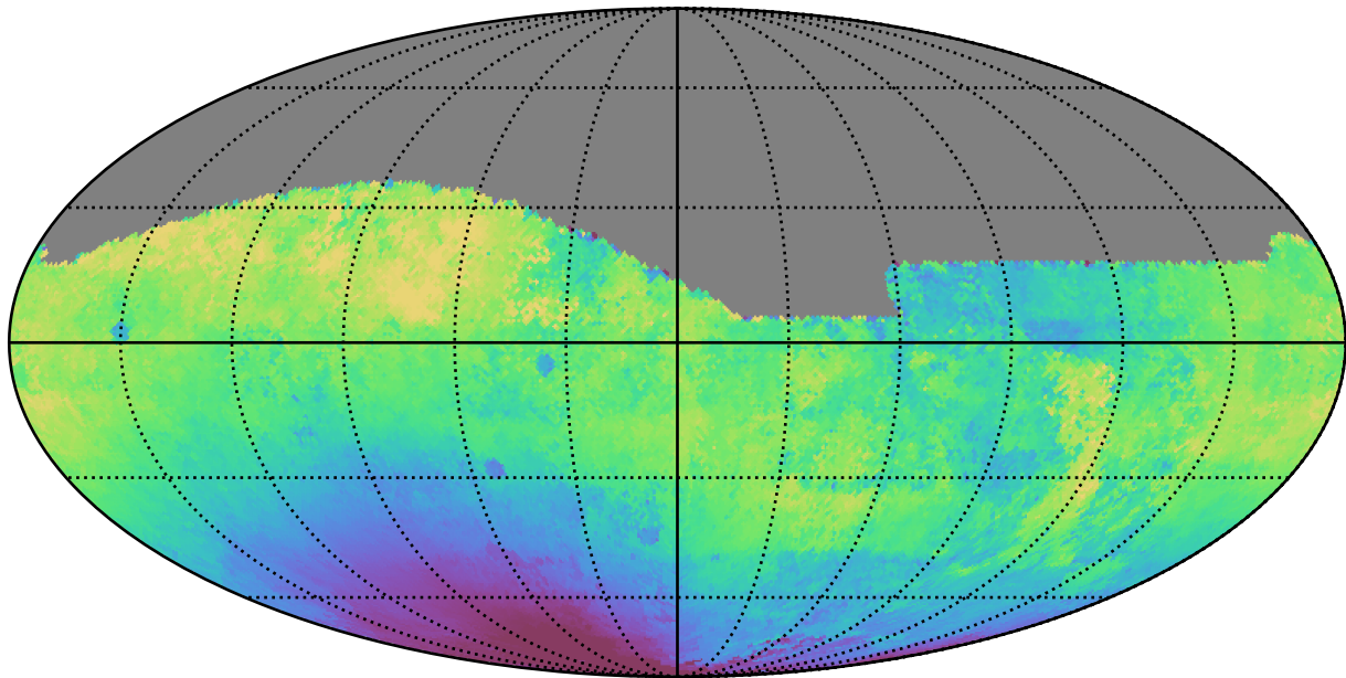
mw_roll_bulge_v3.3_10yrs All sky g band: Median solarElong
