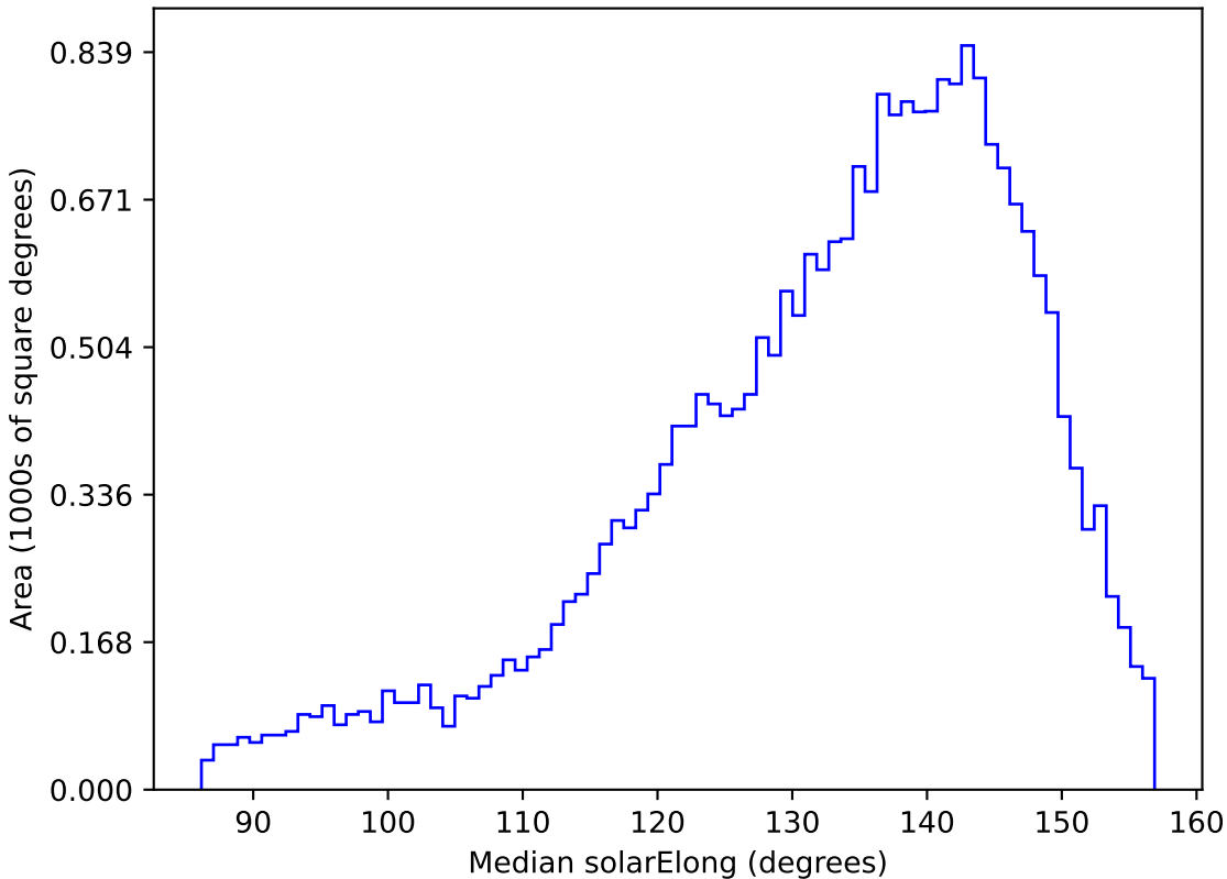
mw_roll_bulge_v3.3_10yrs All sky g band: Median solarElong
