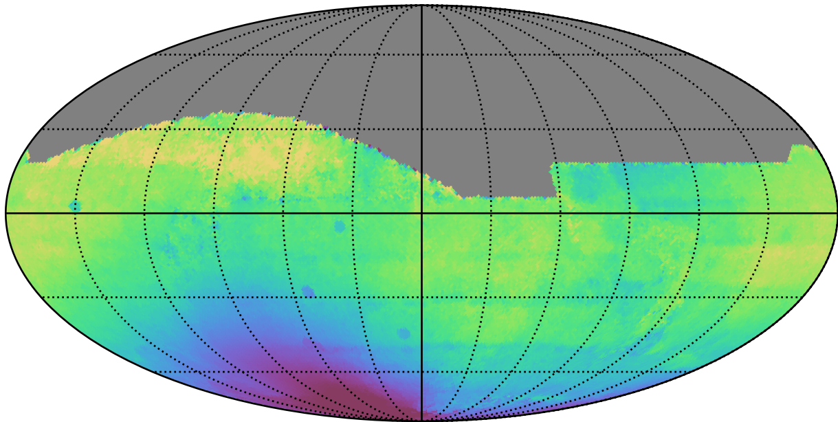
mw_roll_bulge_v3.3_10yrs All sky all bands: Median solarElong
