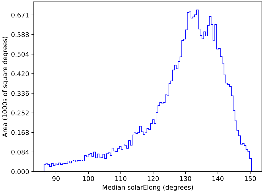
mw_roll_bulge_v3.3_10yrs All sky all bands: Median solarElong
