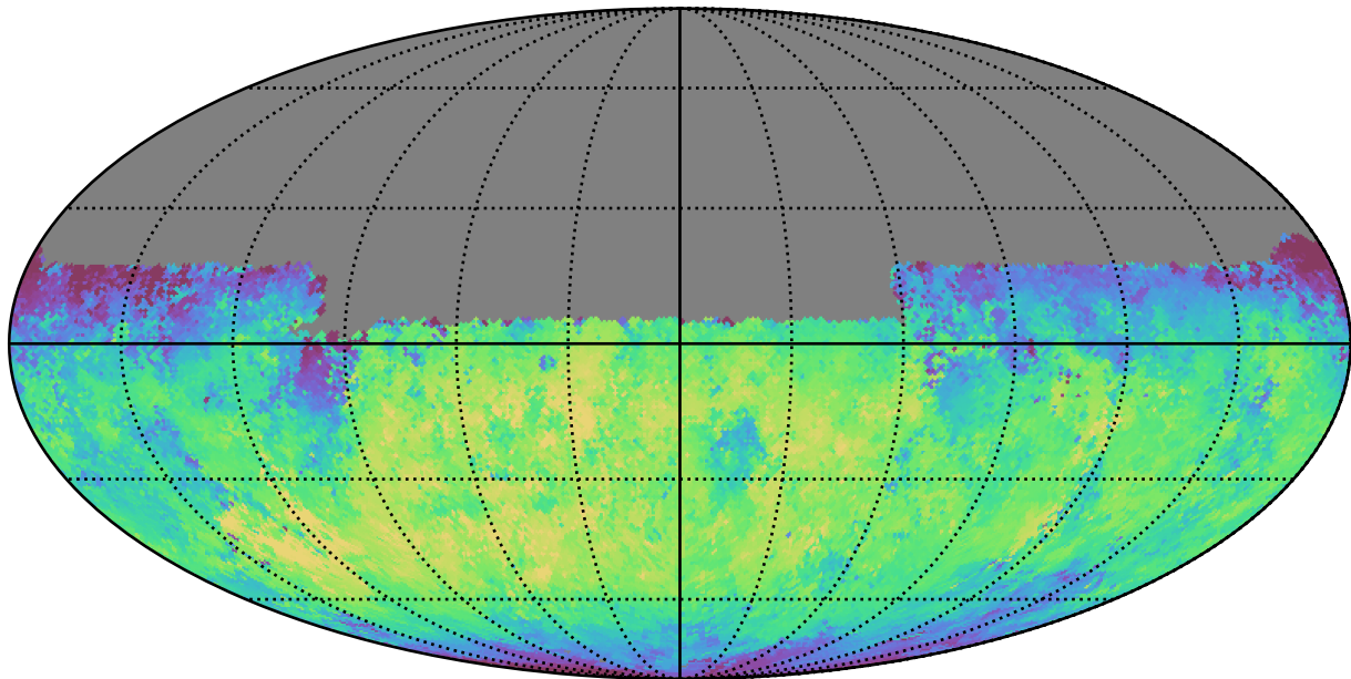
mw_roll_bulge_v3.3_10yrs Yr 1 y band: Median skyBrightness
