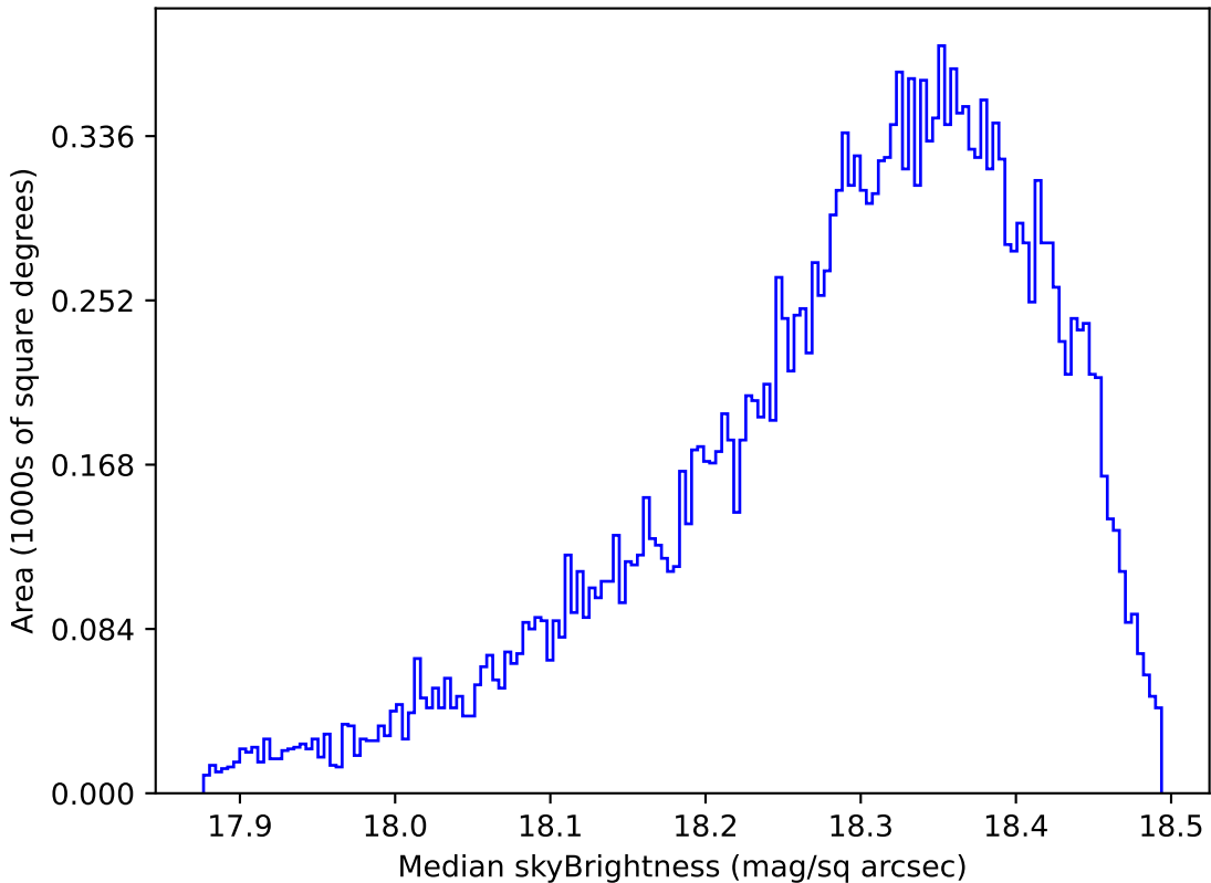
mw_roll_bulge_v3.3_10yrs Yr 1 y band: Median skyBrightness
