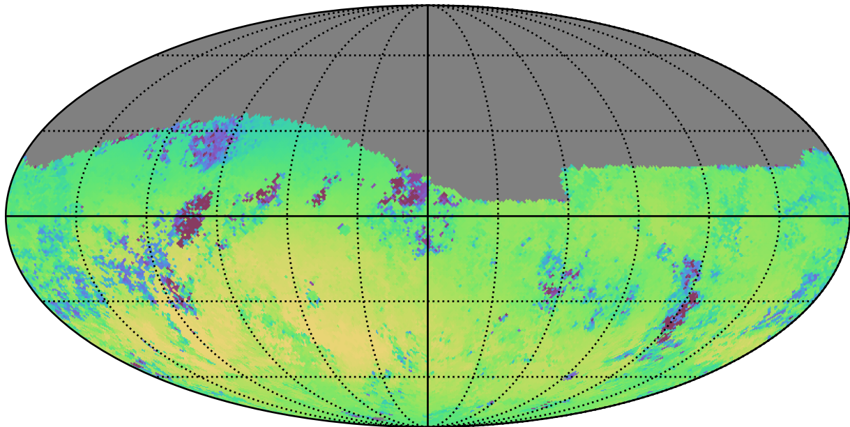
mw_roll_bulge_v3.3_10yrs Yr 1 r band: Median skyBrightness
