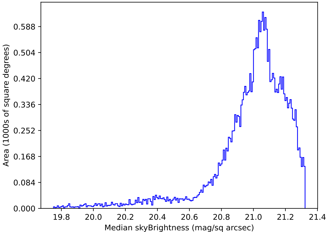
mw_roll_bulge_v3.3_10yrs Yr 1 r band: Median skyBrightness
