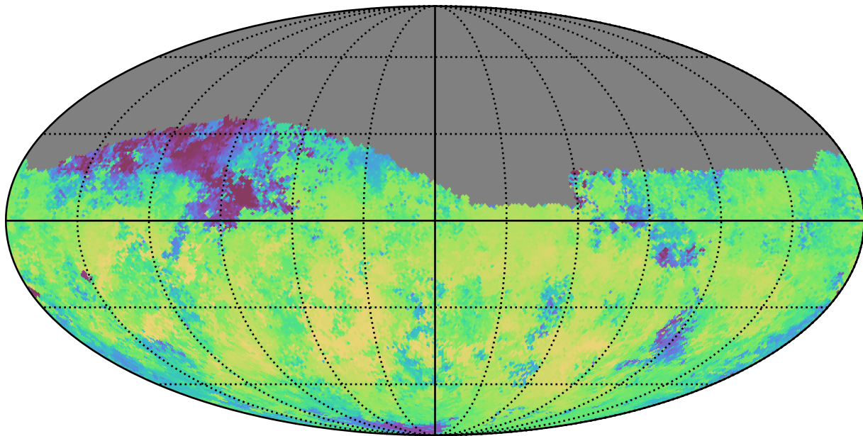
mw_roll_bulge_v3.3_10yrs Yr 1 i band: Median skyBrightness
