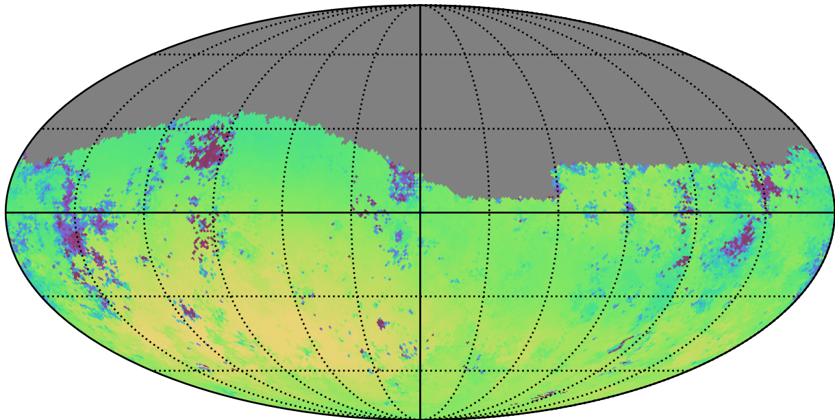
mw_roll_bulge_v3.3_10yrs Yr 1 g band: Median skyBrightness
