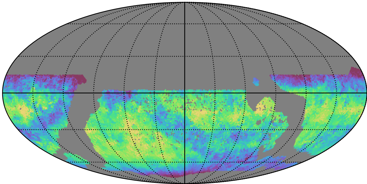
mw_roll_bulge_v3.3_10yrs WFD z band: Median skyBrightness
