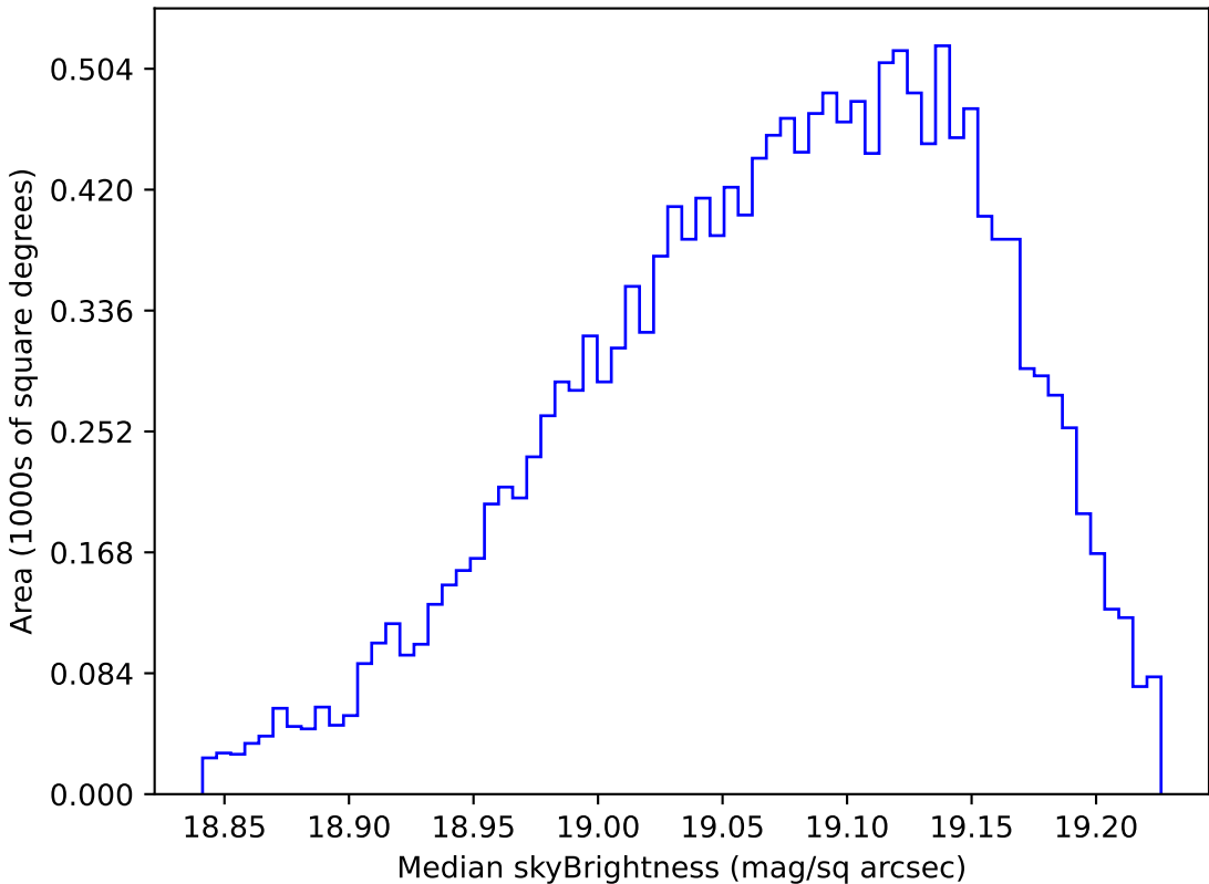
mw_roll_bulge_v3.3_10yrs WFD z band: Median skyBrightness
