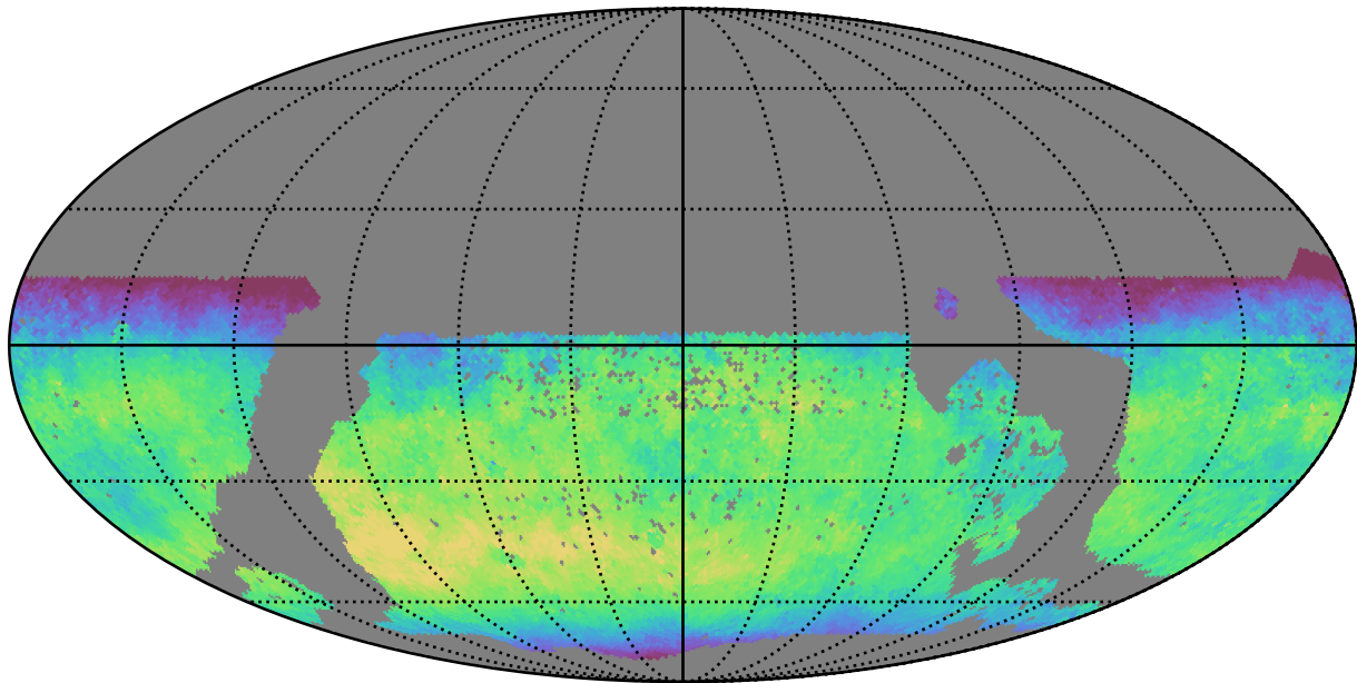
mw_roll_bulge_v3.3_10yrs WFD y band: Median skyBrightness
