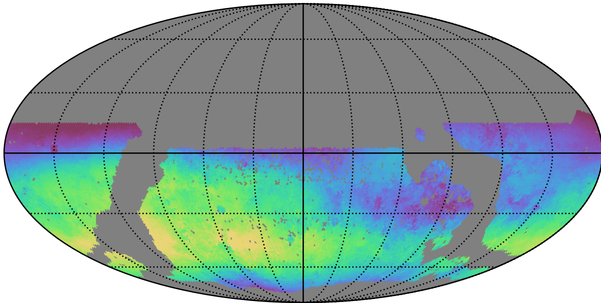
mw_roll_bulge_v3.3_10yrs WFD u band: Median skyBrightness
