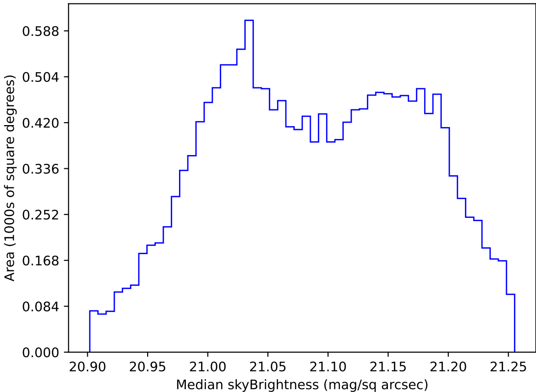
mw_roll_bulge_v3.3_10yrs WFD r band: Median skyBrightness
