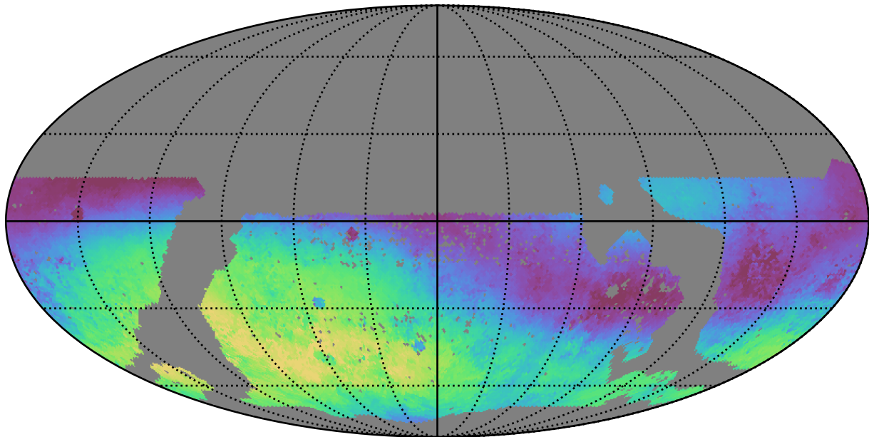
mw_roll_bulge_v3.3_10yrs WFD g band: Median skyBrightness
