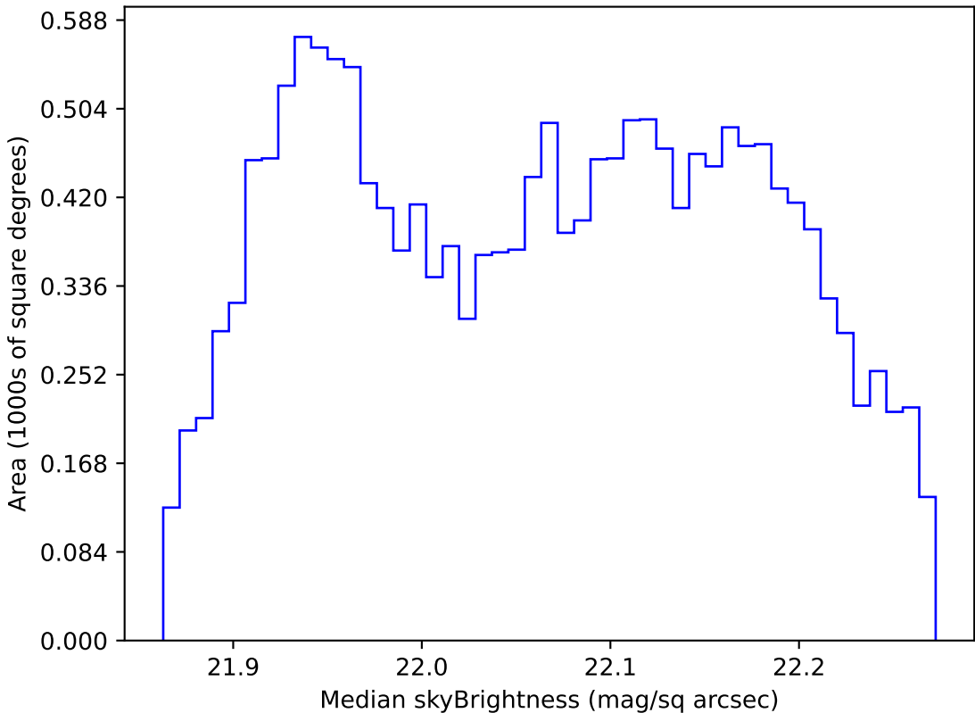
mw_roll_bulge_v3.3_10yrs WFD g band: Median skyBrightness
