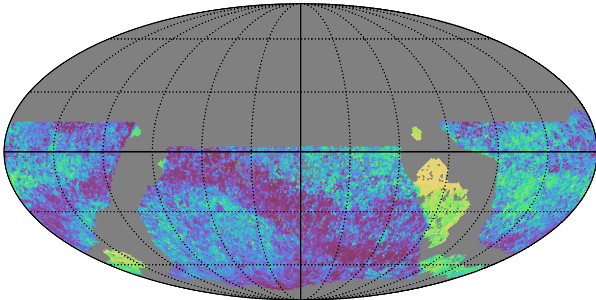
mw_roll_bulge_v3.3_10yrs WFD all bands: Median skyBrightness
