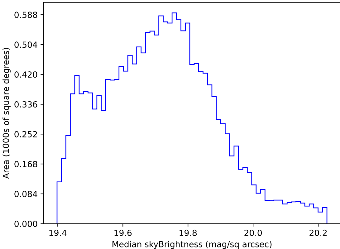
mw_roll_bulge_v3.3_10yrs WFD all bands: Median skyBrightness
