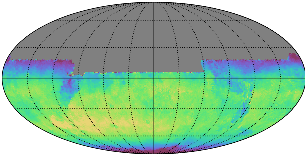
mw_roll_bulge_v3.3_10yrs All sky y band: Median skyBrightness
