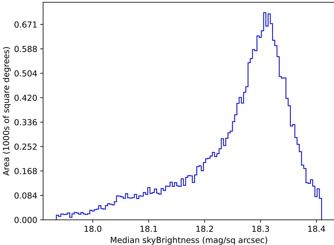
mw_roll_bulge_v3.3_10yrs All sky y band: Median skyBrightness
