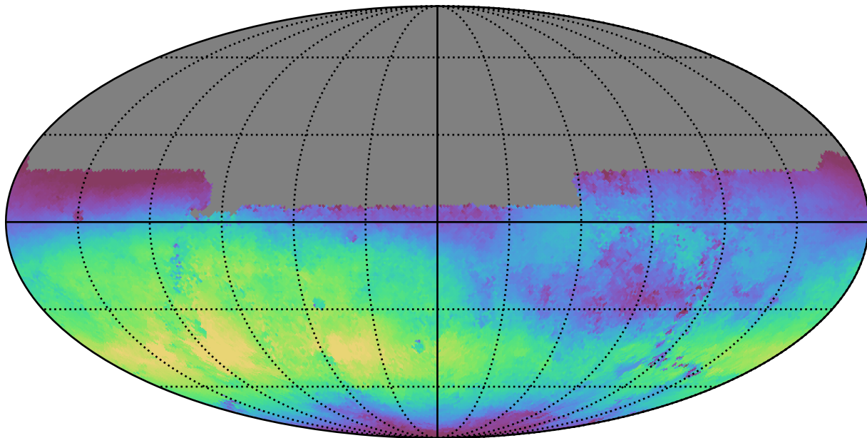
mw_roll_bulge_v3.3_10yrs All sky u band: Median skyBrightness
