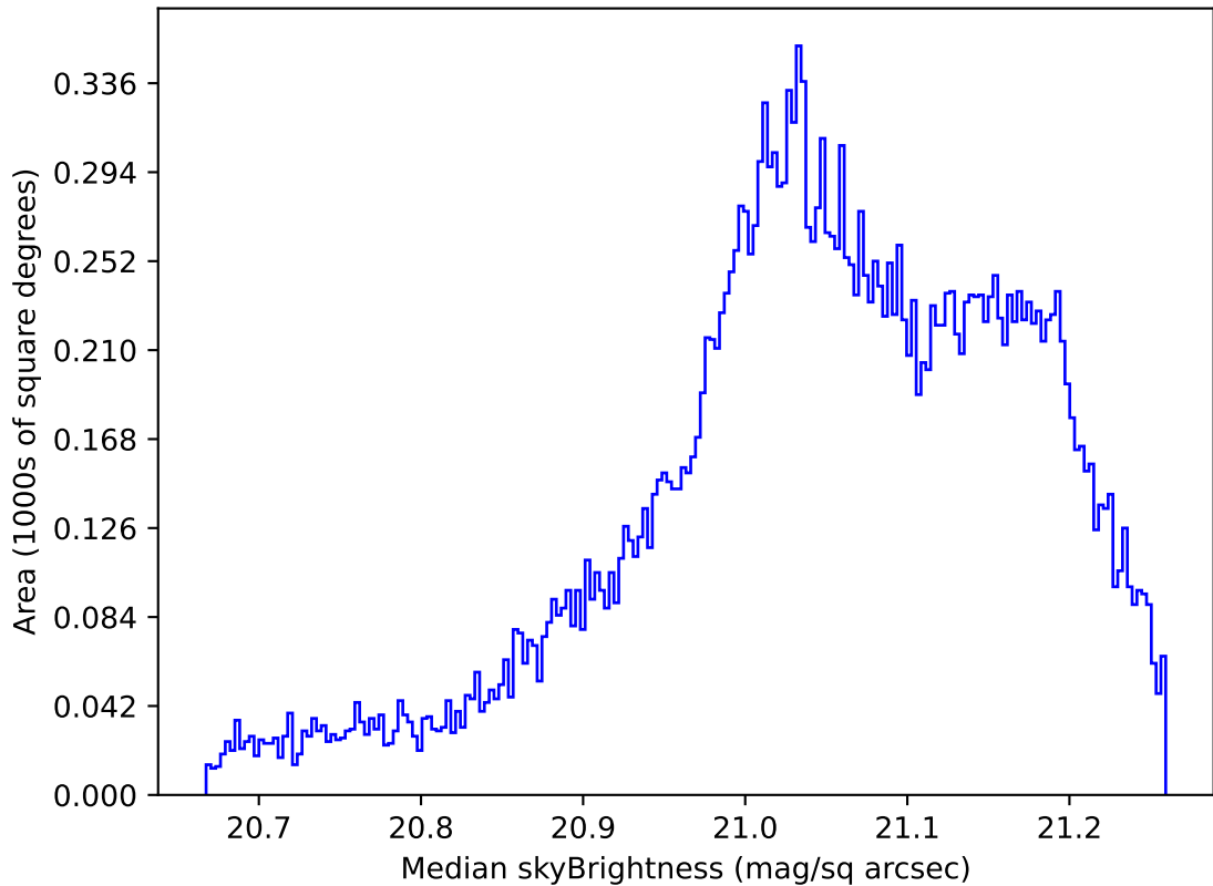
mw_roll_bulge_v3.3_10yrs All sky r band: Median skyBrightness
