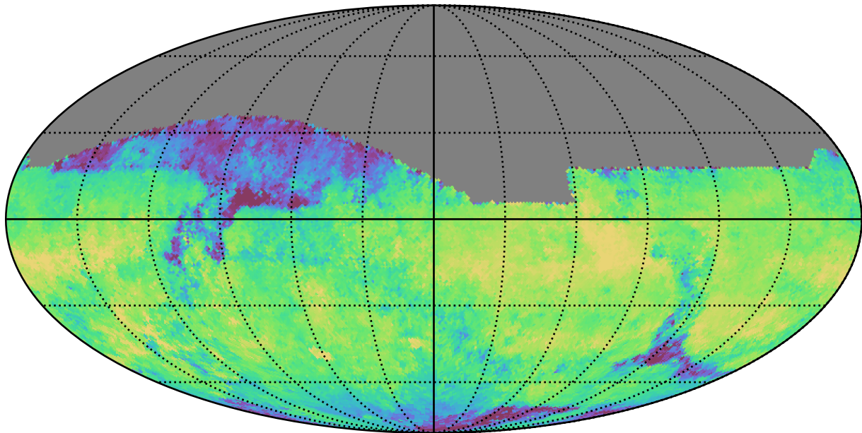
mw_roll_bulge_v3.3_10yrs All sky i band: Median skyBrightness
