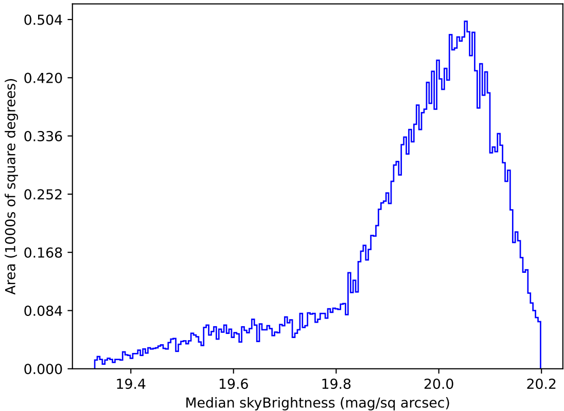
mw_roll_bulge_v3.3_10yrs All sky i band: Median skyBrightness
