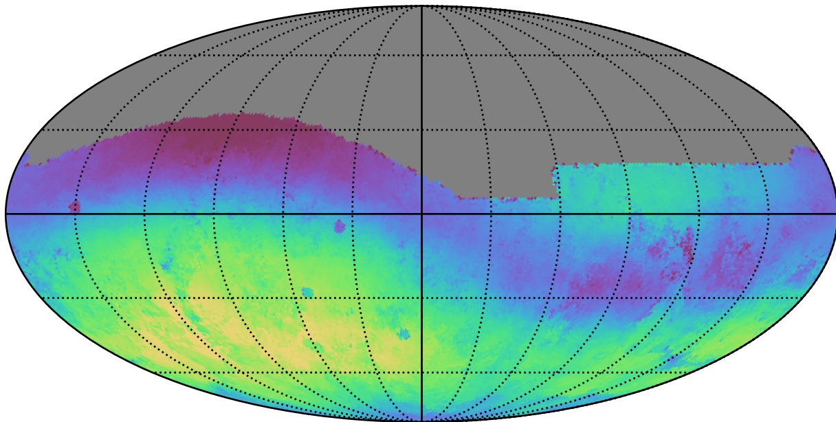
mw_roll_bulge_v3.3_10yrs All sky g band: Median skyBrightness
