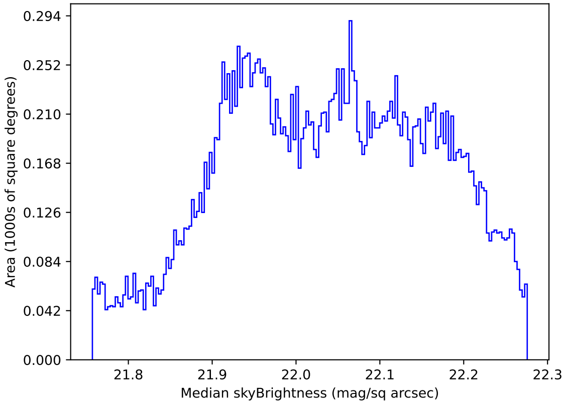
mw_roll_bulge_v3.3_10yrs All sky g band: Median skyBrightness
