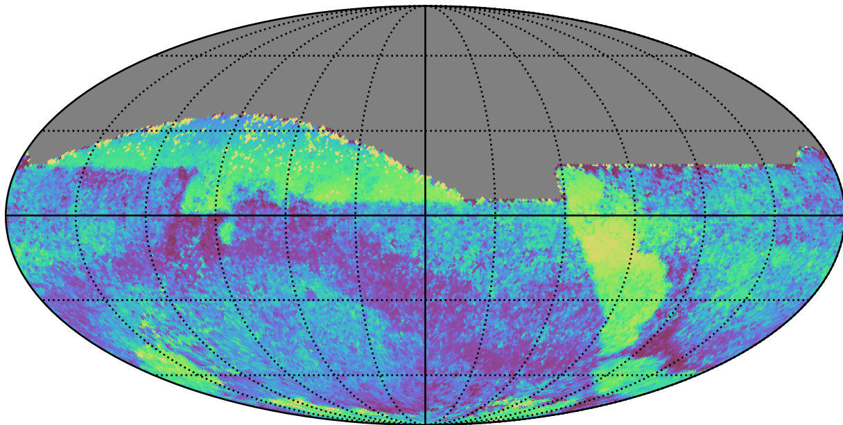
mw_roll_bulge_v3.3_10yrs All sky all bands: Median skyBrightness
