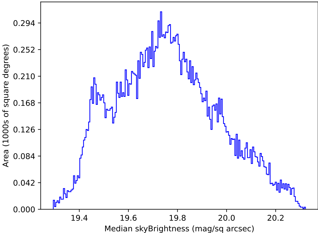
mw_roll_bulge_v3.3_10yrs All sky all bands: Median skyBrightness
