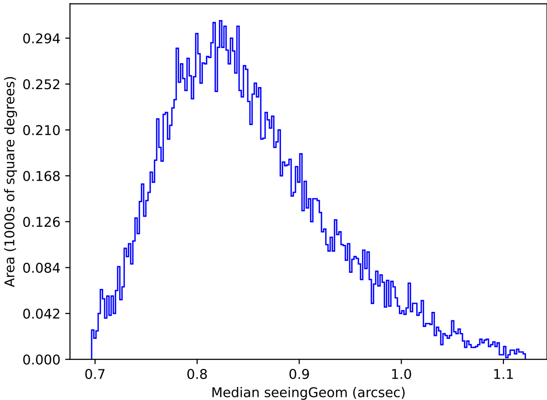
mw_roll_bulge_v3.3_10yrs Yr 1 y band: Median seeingGeom
