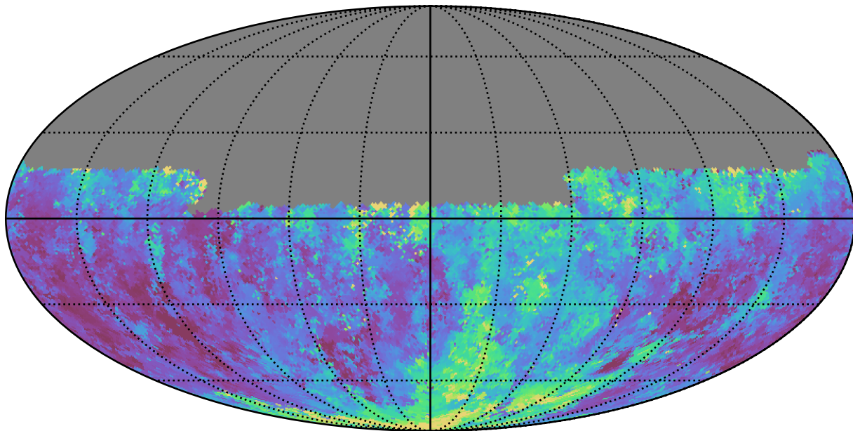
mw_roll_bulge_v3.3_10yrs Yr 1 u band: Median seeingGeom
