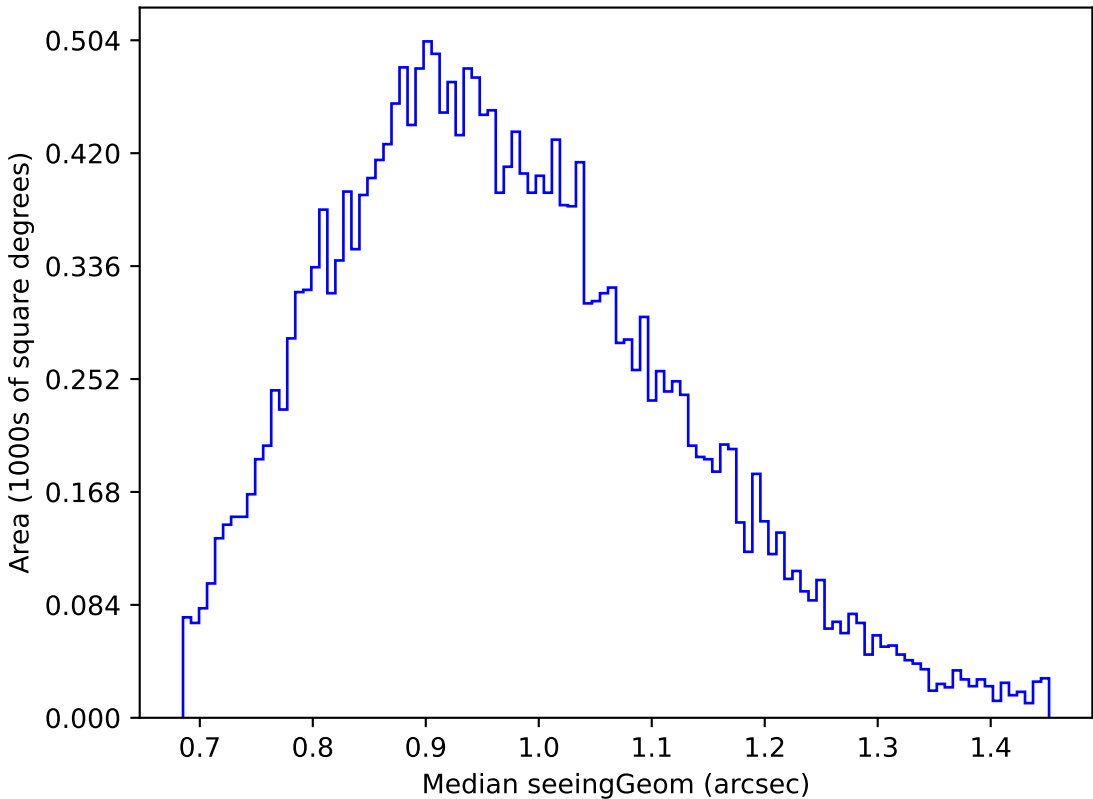
mw_roll_bulge_v3.3_10yrs Yr 1 u band: Median seeingGeom
