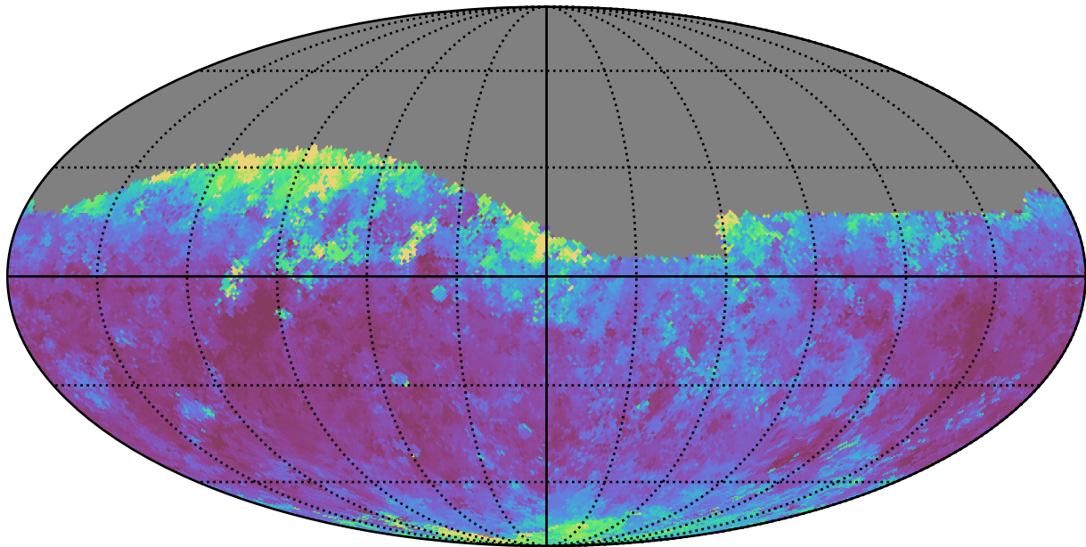
mw_roll_bulge_v3.3_10yrs Yr 1 r band: Median seeingGeom
