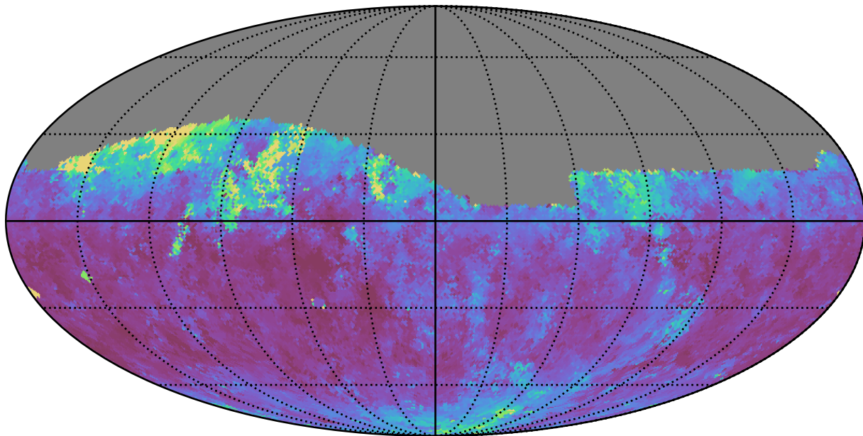
mw_roll_bulge_v3.3_10yrs Yr 1 i band: Median seeingGeom
