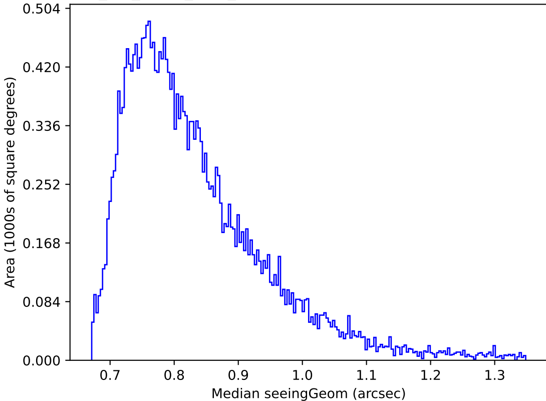
mw_roll_bulge_v3.3_10yrs Yr 1 i band: Median seeingGeom
