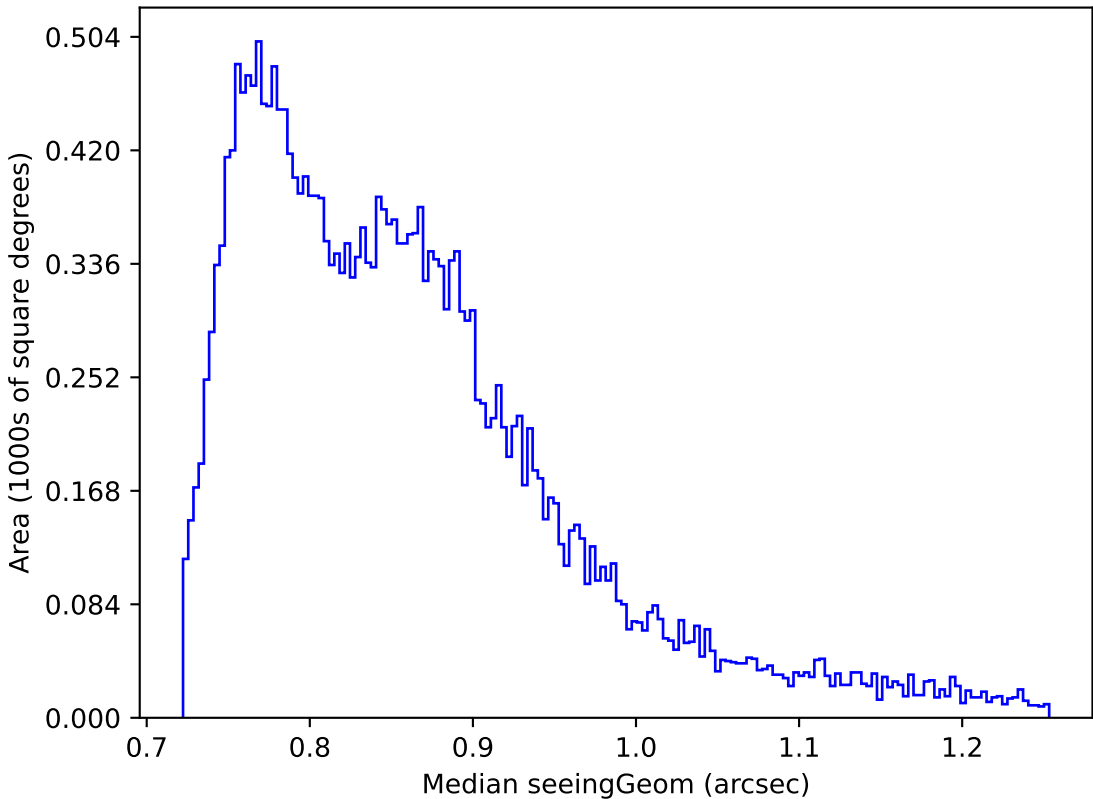
mw_roll_bulge_v3.3_10yrs Yr 1 all bands: Median seeingGeom
