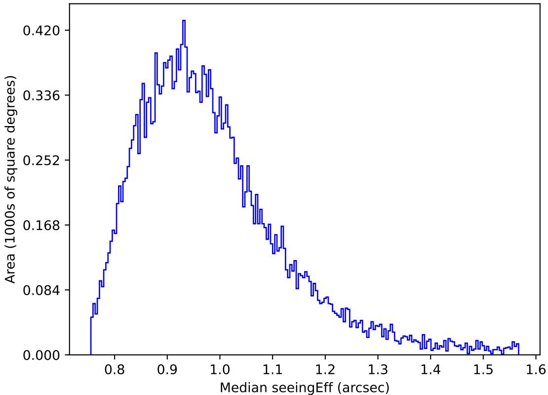
mw_roll_bulge_v3.3_10yrs Yr 1 z band: Median seeingEff
