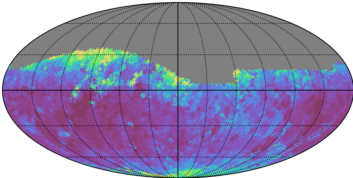
mw_roll_bulge_v3.3_10yrs Yr 1 r band: Median seeingEff
