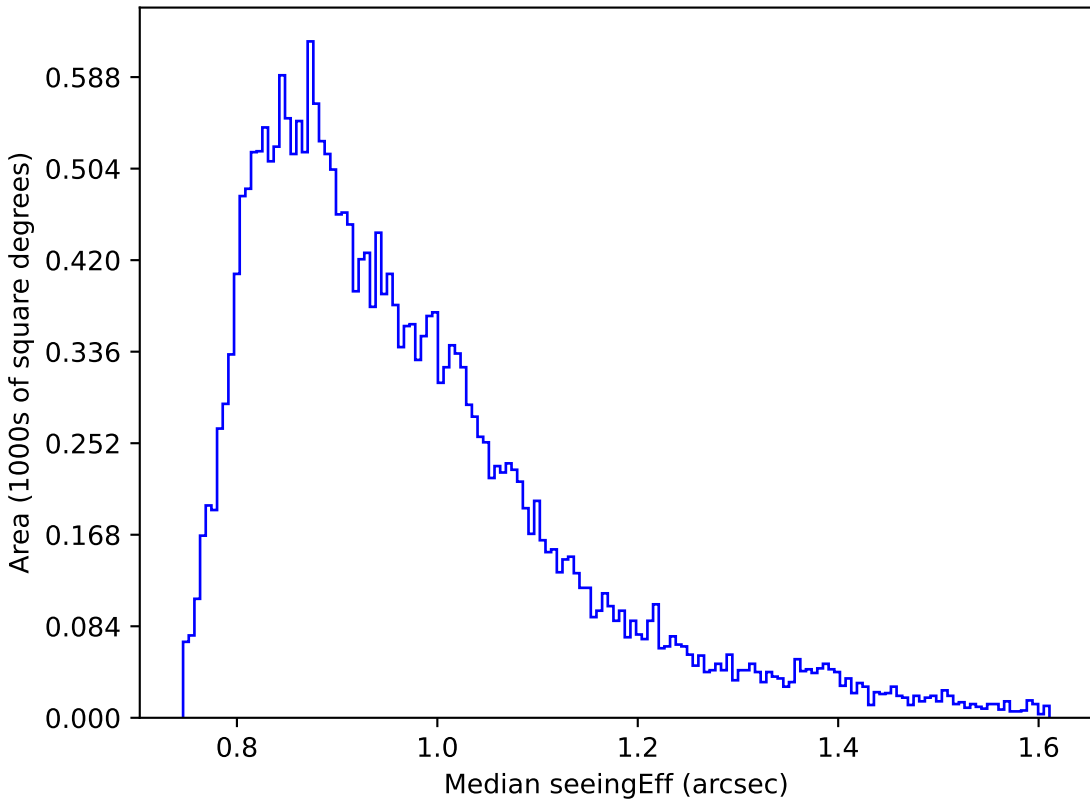
mw_roll_bulge_v3.3_10yrs Yr 1 r band: Median seeingEff
