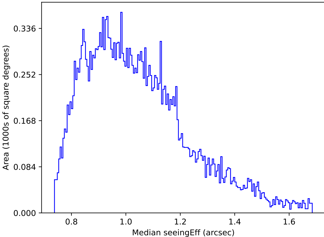
mw_roll_bulge_v3.3_10yrs Yr 1 g band: Median seeingEff
