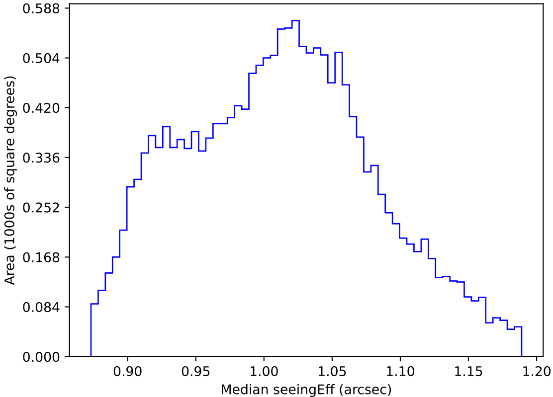
mw_roll_bulge_v3.3_10yrs WFD z band: Median seeingEff
