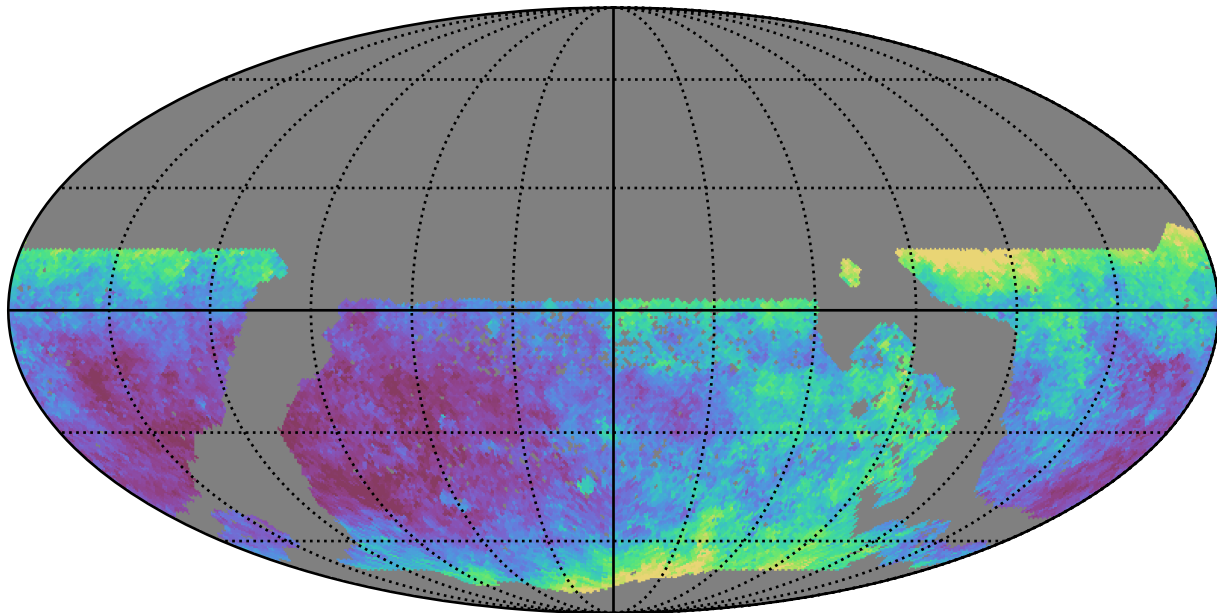
mw_roll_bulge_v3.3_10yrs WFD y band: Median seeingEff
