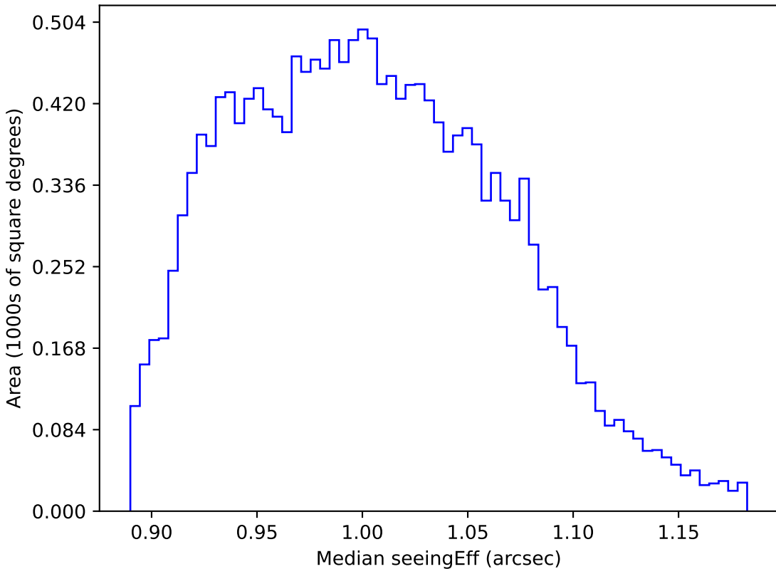
mw_roll_bulge_v3.3_10yrs WFD y band: Median seeingEff
