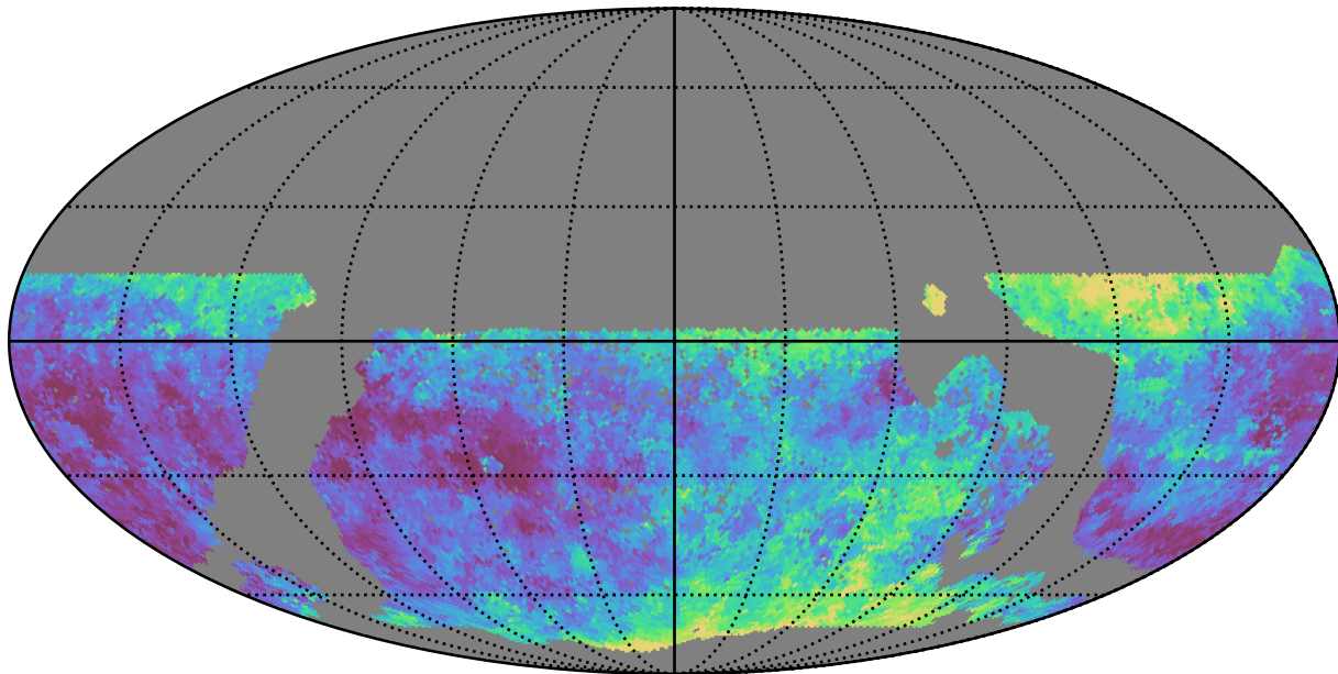
mw_roll_bulge_v3.3_10yrs WFD u band: Median seeingEff
