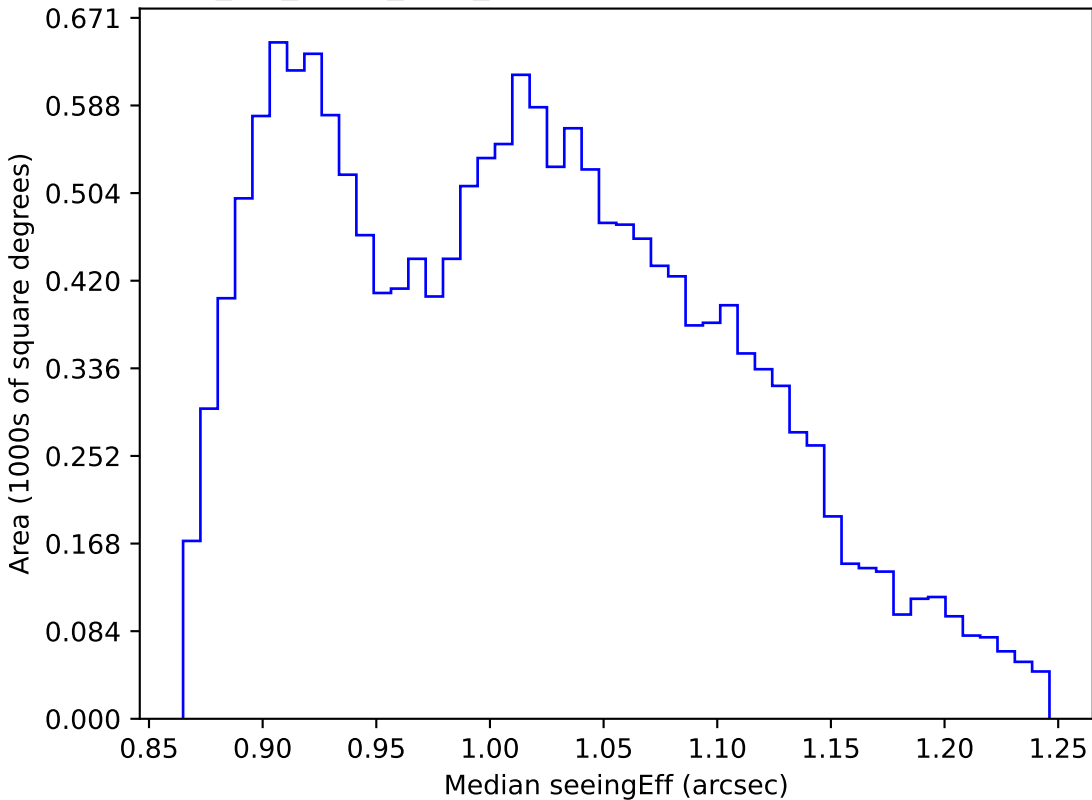
mw_roll_bulge_v3.3_10yrs WFD r band: Median seeingEff
